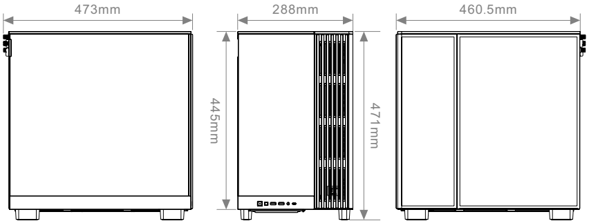
Chassis dimension
