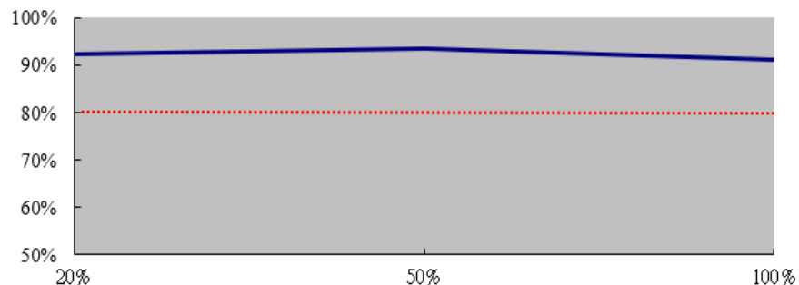
Efficiency of the Power Supply
