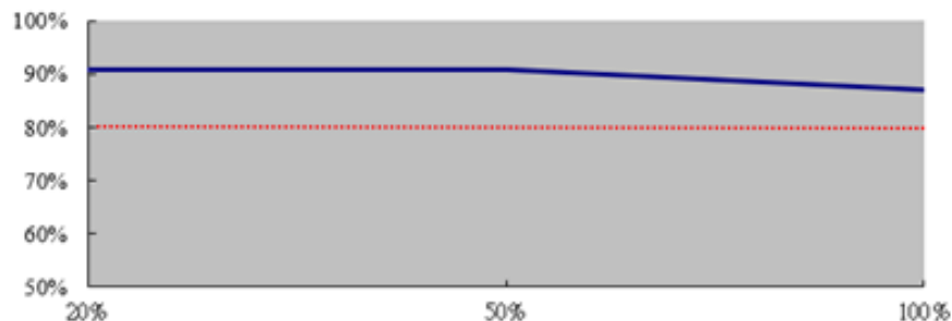
Efficiency of the Power Supply
