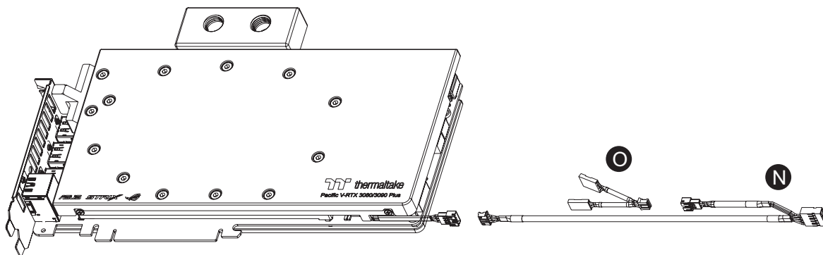
Connect the MB SYNC Cable to Water block
