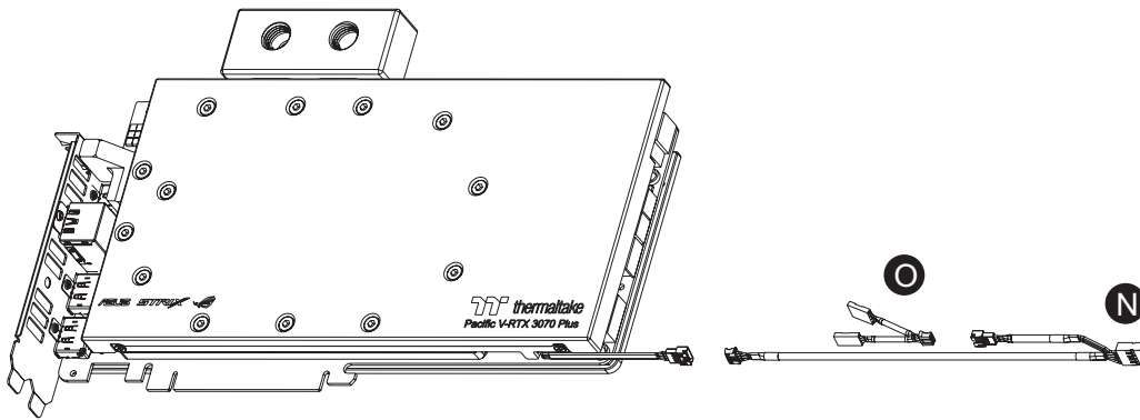
Connect the MB SYNC Cable to Water block
