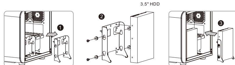
3.5" HDD
