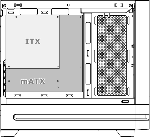
Motherboard Compatibility: ITX / mATX
