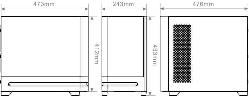
Chassis dimension
