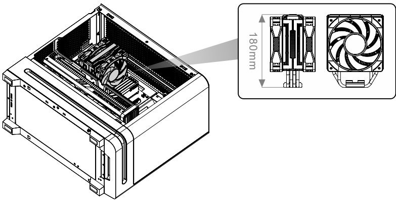
CPU cooler max height: 180mm
