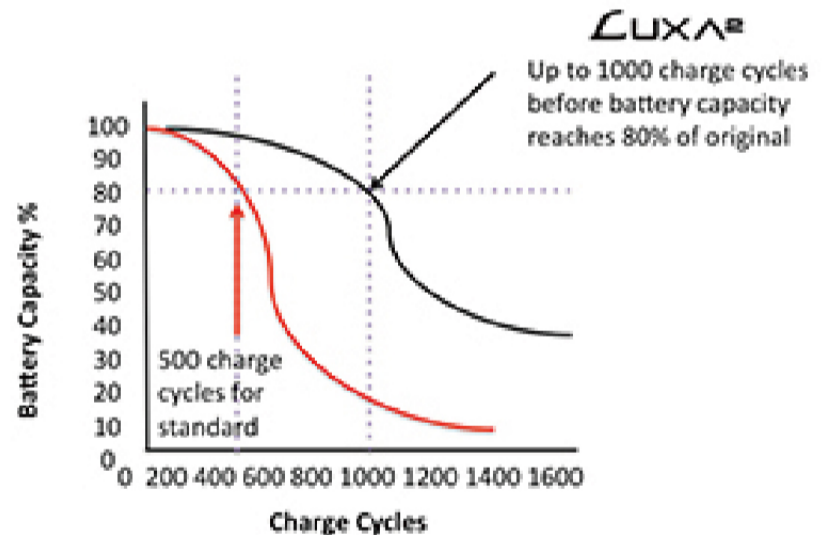
7 LUXA2 charge cycle comparison graph.
