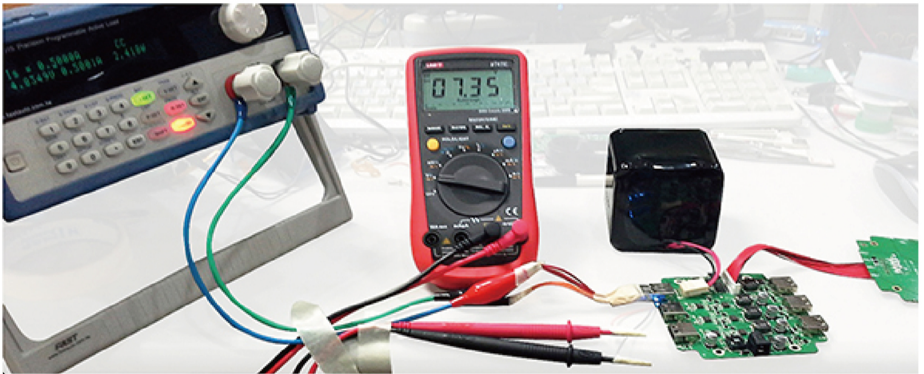
6.1 Input testing in progress.
